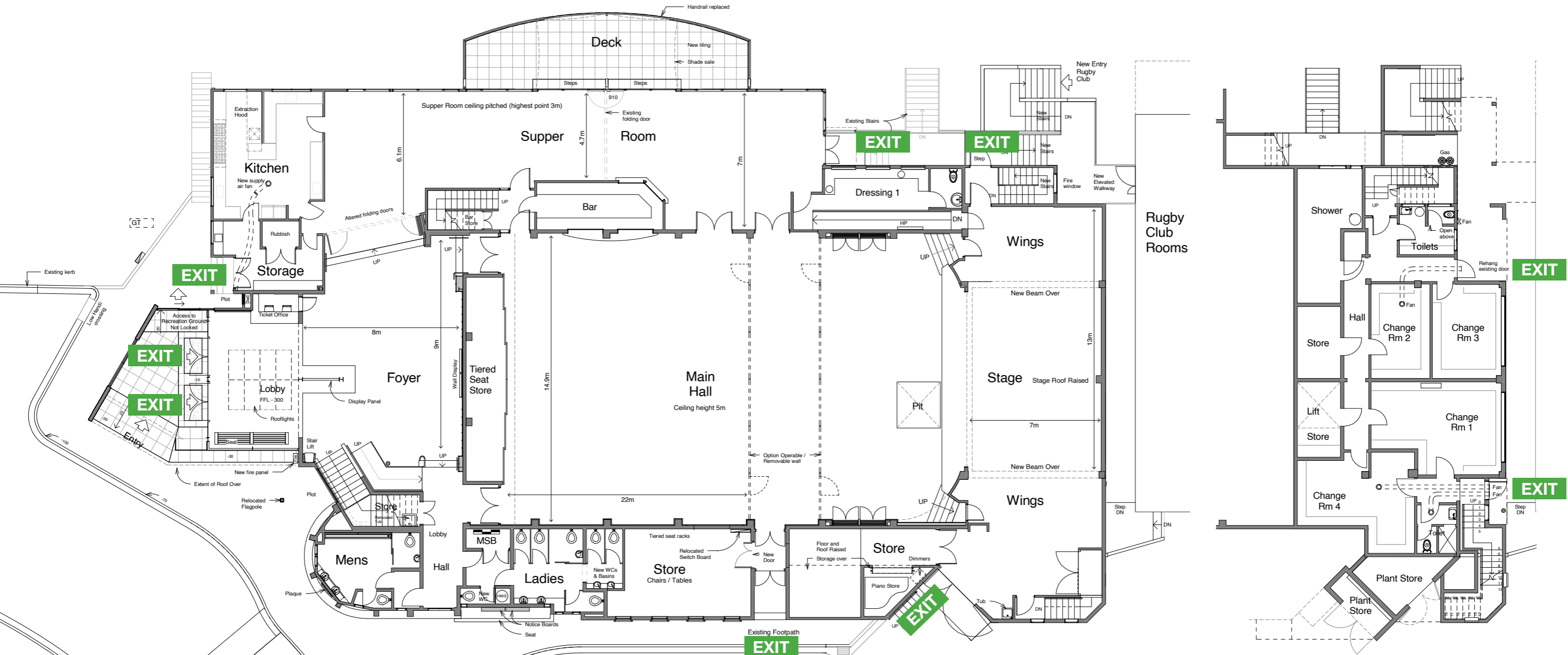
1 Hall Plan
