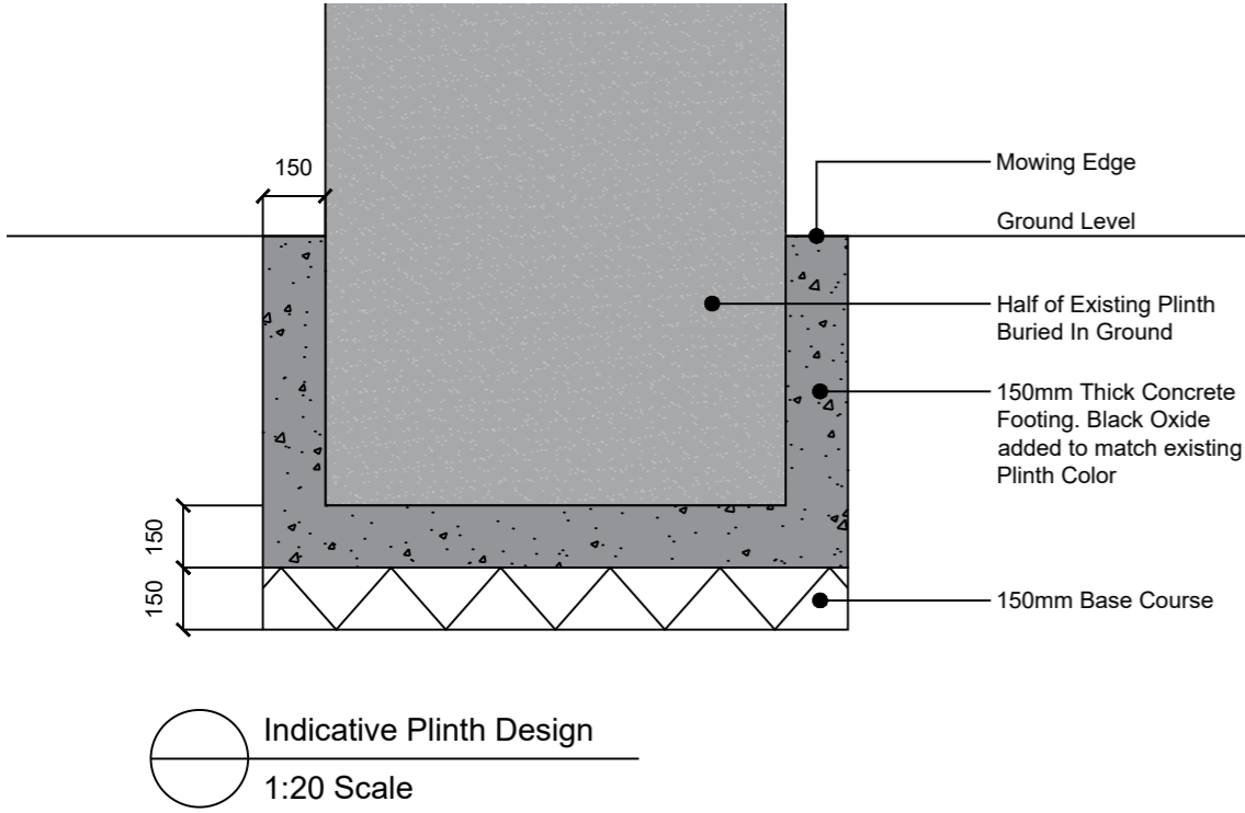
Plinth Detail
