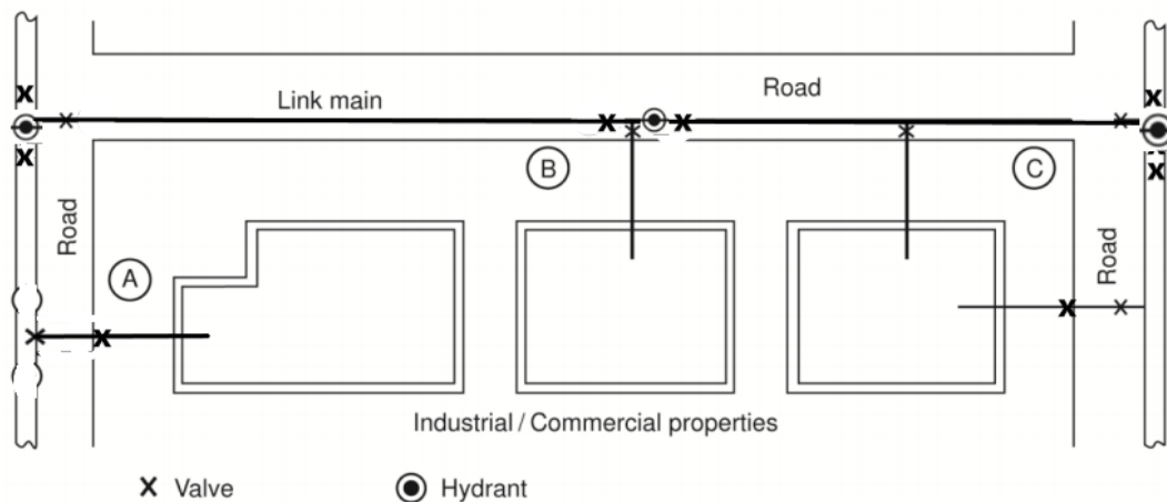
Figure 6.3 – Secure connection
